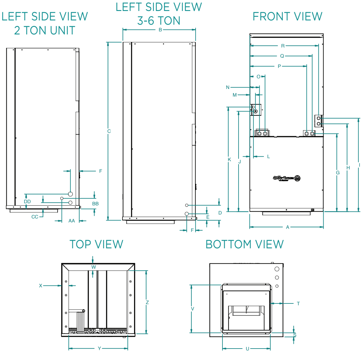
SAH Air Handler - Bottom flow
