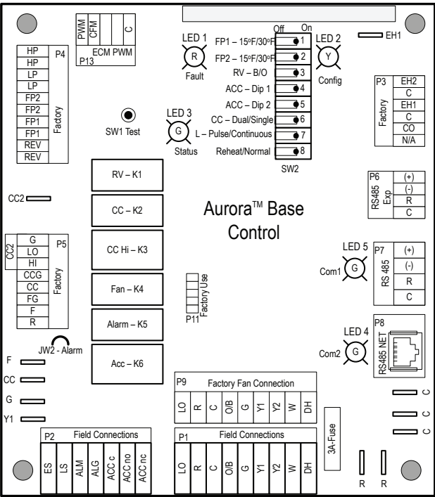
ABC Control Board Layout
