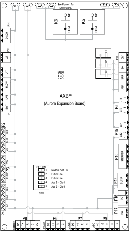
AXB Control Board Layout
