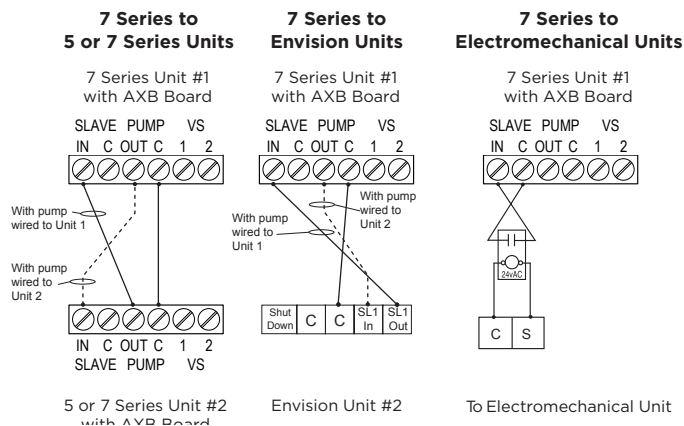
Figure 8: Primary/Secondary Hook-up
