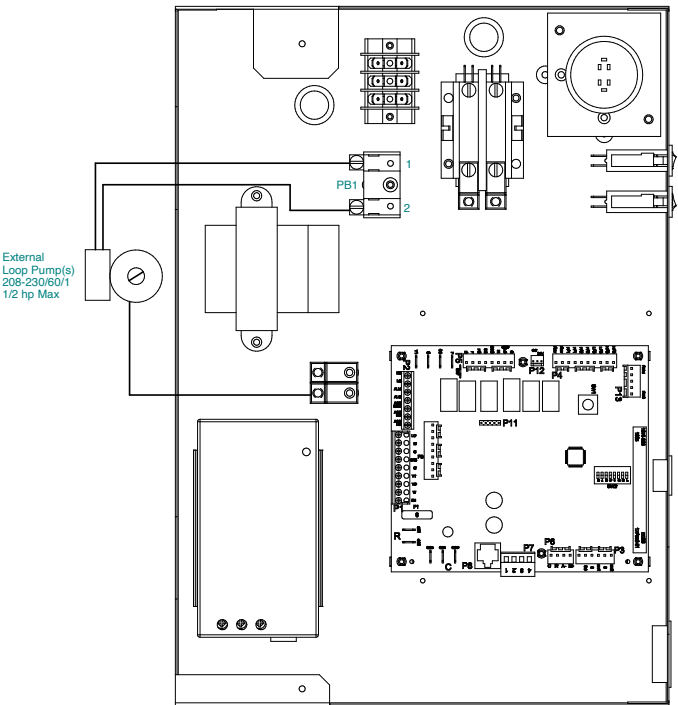
Figure 14: Pump Wiring 208-230/60/1
