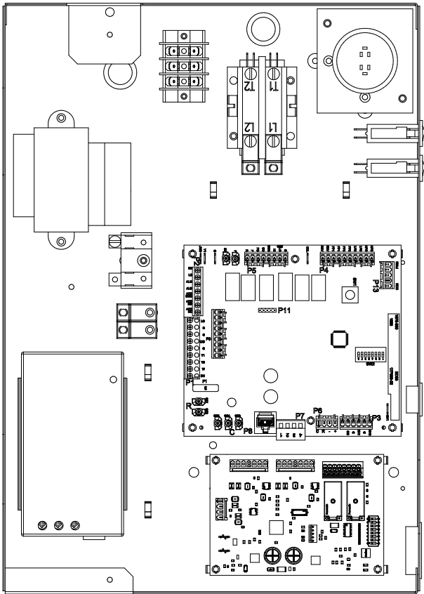
Figure 13C: Control Box with ASB Board
