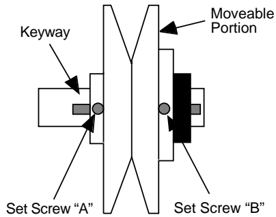
Figure 10: Blower Motor Sheave Adjustments and Settings
