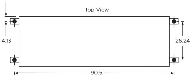
Figure 2: Mounting Rod Layout
