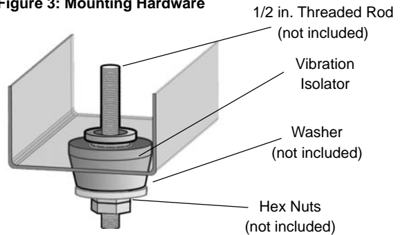
Figure 3: Mounting Hardware
