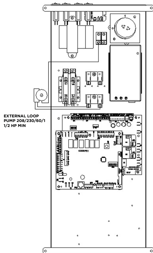
Figure 5: Source Pump Wiring 208-230/60/1
