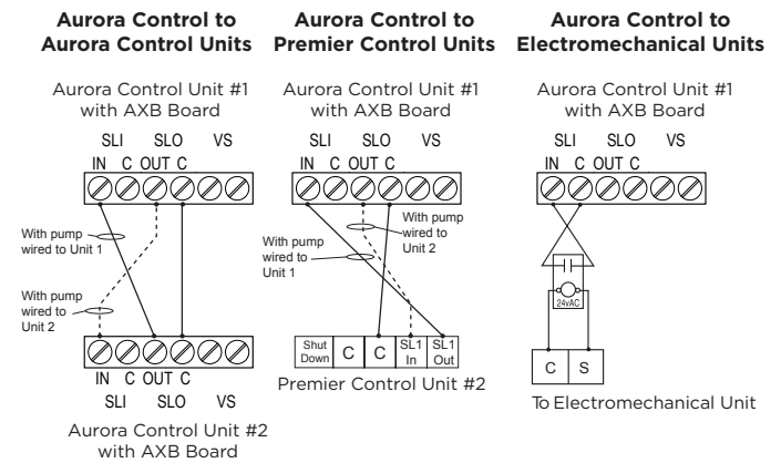
Figure 2: Primary/Secondary Hook-up
