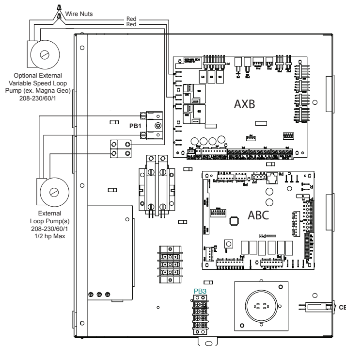
Figure 14: Pump Wiring 208-230/60/1
