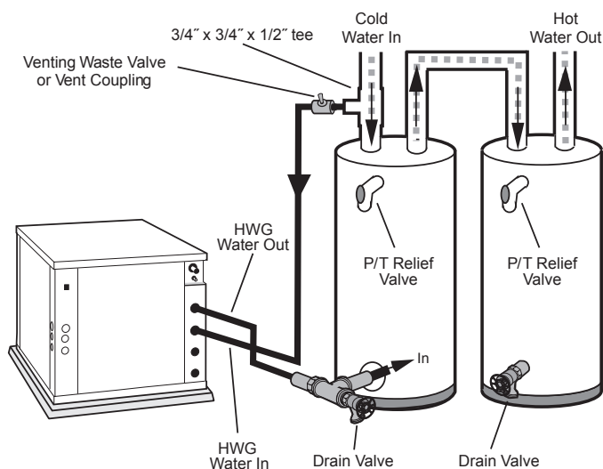
Figure 9: Hot Water Generator Installation in Preheat Tank
