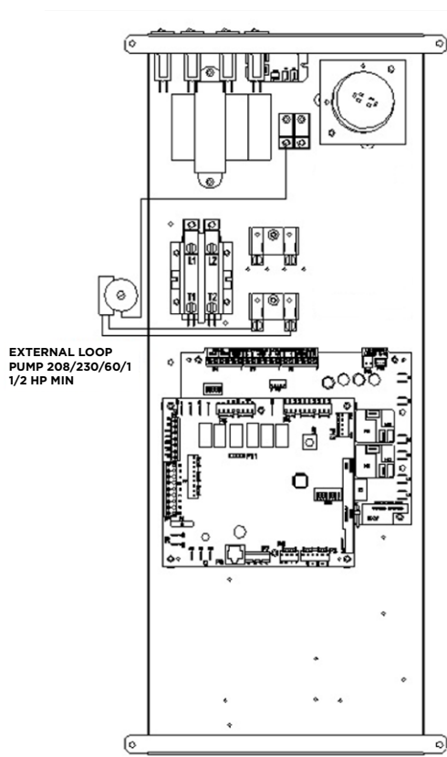
Figure 5: Source Pump Wiring 208-230/60/1
