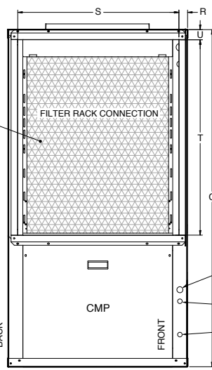
LEFT VIEW - LEFT RETURN
